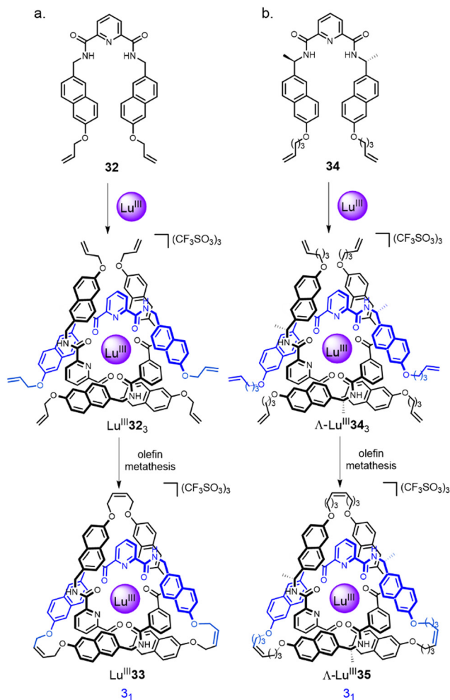
Fig. 11 Synthesis of: (a) trefoil knot \text{Lu}^{\text{III}}\mathbf{33} via racemic circular helicate \text{Lu}^{\text{III}}\mathbf{32}_3 , 20 (b) trefoil knot \Lambda\text{-Lu}^{\text{III}}\mathbf{35} via enantiopure circular helicate \Lambda\text{-Lu}^{\text{III}}\mathbf{34}_3 . 70
