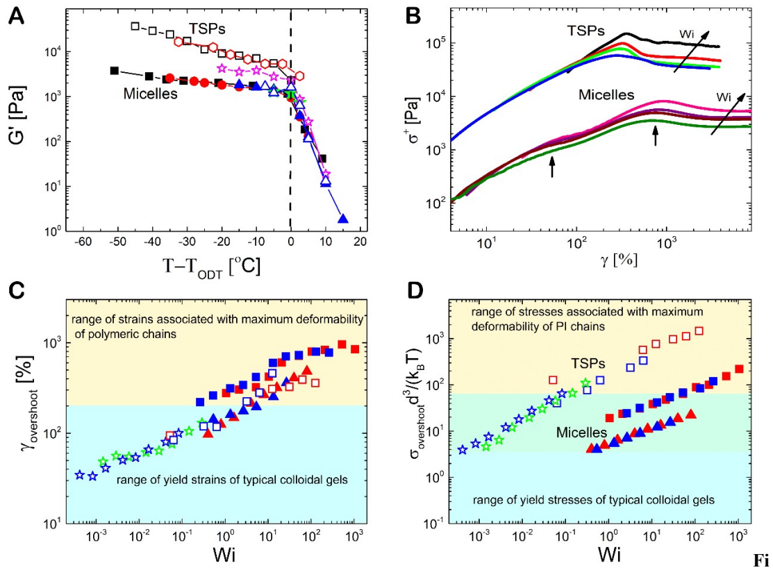
Figure 6. Rheological properties of TSPs and micelles in the concentrated regime: (A) Storage modulus G' measured at a frequency of \omega=1\text{rad/s} as a function of the distance from the order to disorder transition (ODT) for micelles (closed symbols) and TSPs (open symbols) at concentrations of 40%w/w (square symbols), 37% w/w (diamond symbols), 33%w/w (star symbols), 30%w/w (triangle symbols) and 27%w/w (circle symbols). (B) Start-up shear flow experiments performed at different
