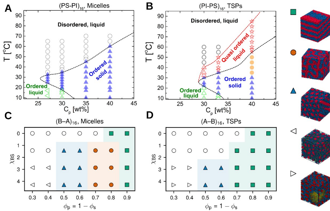
Figure 4. Tentative phase diagrams from experiments and simulations: (A) and (B): Experimental phase diagrams of the star block copolymer with sticky PS blocks as the inner (A) and outer (B) blocks. The black dashed curve is a guide to the eye and the region inside corresponds to a solid-like response (closed symbols) characterized by G' > G'' , whereas the area outside features a liquid-like response (open symbols). The red and black dashed curves in (B) define a region of quasi-ordered liquid arrangement at high temperatures. Symbols illustrate the phases obtained from SAXS: disorder (circles), hexagonally packed cylinders (blue and green top-pointing triangles), cubic phase (green left-pointing triangles), textured double diamond (stars) and gyroids (orange circles). (C) and (D): Phase diagrams in simulations as obtained for model star block copolymers in solution with the inner (C) and outer (D) sticky blocks, as a function of varying incompatibility parameter \chi_{BS} and the polymer volume fraction \phi_p . Note that the vertical axes in (C) and (D) are inverted ( \chi_{BS} values grow from top to bottom), to match the trend with T in experiments. The phase diagrams in (C) and (D) were obtained for \chi_{AS} = 0 , corresponding to experimental phase diagrams (A) and (B) for T > T_{PI}^{\theta} . The snapshots on the right-hand side illustrate the phases obtained in the simulations: lamellae (green squares), gyroids (orange circles), system-spanning cylinders (blue top-pointing triangles). Partly-ordered states with absent long-range order are shown with open triangles: connected bulky cylinders (open left-pointing triangles) and cylinders partly phase-separated from the solvent (open right-pointing triangles; the
