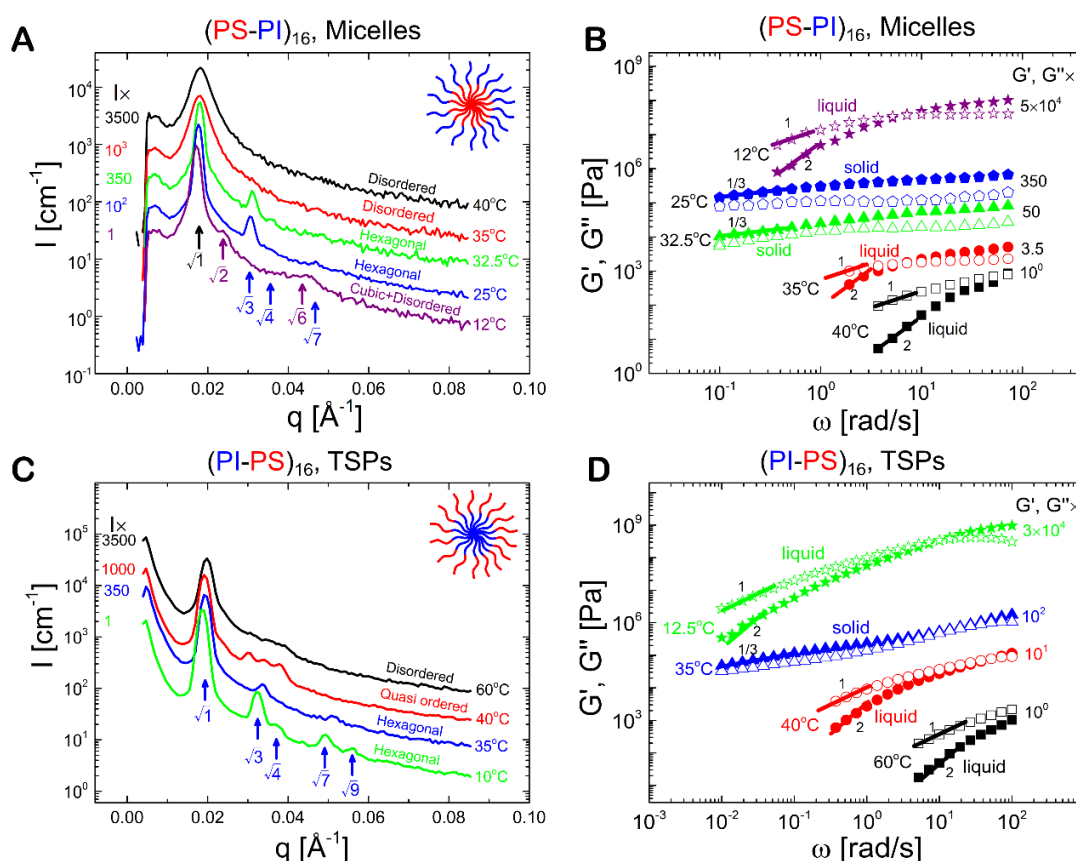
Figure 2. Structural and rheological properties of star block copolymers in concentrated regime:
