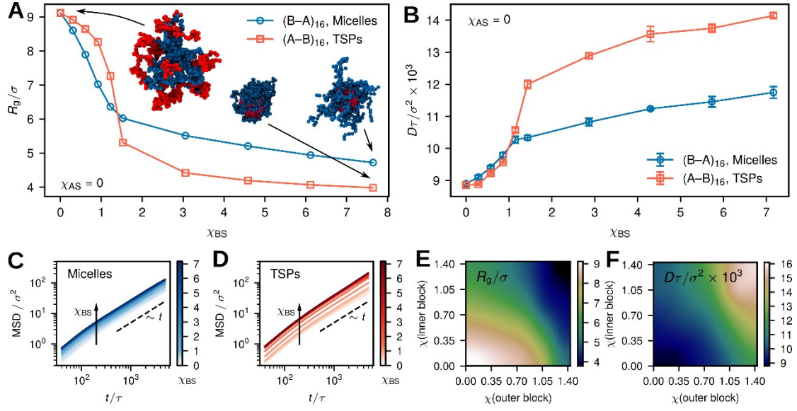
Figure 1. Conformations and dynamics of single stars: (A) The radius of gyration R_g of a single star as a function of the incompatibility parameter \chi_{BS} between the solvent and B monomers for the micellar, (B-A)_{16} , (blue open circles) and telechelic, (A-B)_{16} , (red open squares) architectures. The snapshots in (A) indicate typical star conformations with red monomers corresponding to B blocks and blue monomers to A blocks: a telechelic (A-B)_{16} star polymer (TSP) in good solvent conditions (left), a collapsed TSP (center), a collapsed (B-A)_{16} micelle (right). (B) The corresponding center-of-mass diffusion coefficient D for varying \chi_{BS} , as extracted from the mean-square displacements of the star's center of mass for the micellar (C) and telechelic (D) architectures. The A monomers in (A), (B), (C), and (D) are in good solvent conditions with \chi_{AS}=0 . A generic two-dimensional phase diagram for single star's R_g (E) and D (F) in the case of varying incompatibility parameter between the solvent and inner, \chi (inner block), and outer, \chi (outer block) blocks. In all simulations here, we used the value \chi_{AB}=1.03 that corresponds to the experimental PS-PI copolymer within the relevant range of temperatures (see Methods ). The values of the diffusion coefficient were corrected for finite-size effects (see Methods ).
