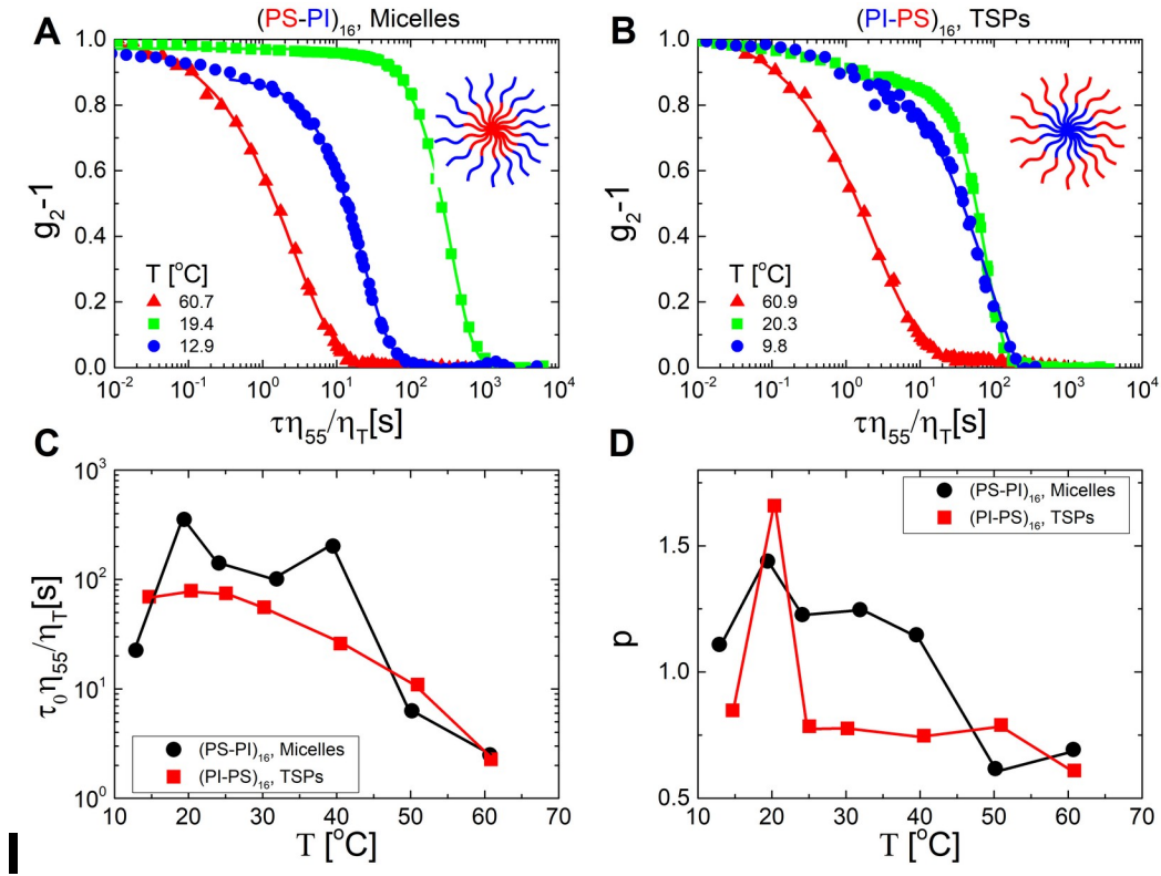
Figure 3. Microscopic dynamics of star block copolymers in the concentrated regime: Representative intensity correlation functions g_2-1 measured at a wavevector q = \hat{i} 24.7 \mu\text{m}^{-1} at different temperatures (shown in the legend) for the micellar (A) and TSPs (B) systems. The solid lines in (A) and (B) represent stretched exponential functions fits. (C) Temperature dependence of the relaxation time of g_2-1 as obtained from stretched exponential fits. (D) Same as in (C), but for the stretching exponent p . In both systems, the star concentration is 30% w/w. In panels (A)-(C), time delays have been normalized to account for the change of solvent viscosity, \eta_T , with temperature. The solvent viscosity at T = \hat{i} 55^\circ\text{C} , \eta_{55} , is taken as a reference value (it corresponds to homogeneous regime, above the cloud point of the PS block). The temperature dependence of solvent viscosity is shown in Fig. S13. In panels (C)-(D) the error bars as determined from the fitting routine are not plotted as they are smaller than or comparable to the symbol size: the percentage errors on time and p (panels C and D, respectively) are smaller than 5.6% and 3.6%.
